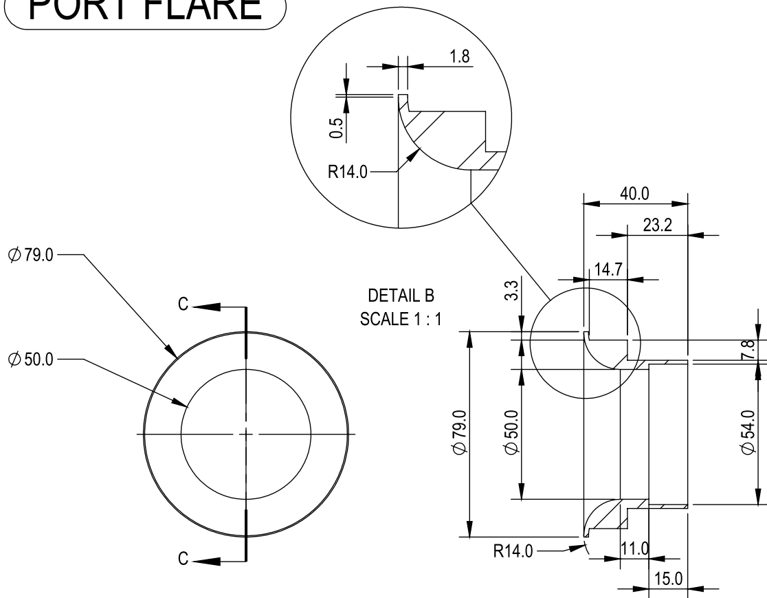
SECTION C-C
